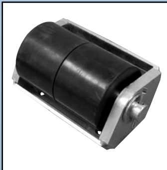
Rubber bumper roll fender Galvanized 195 x 113 mm Roll diameter Ø100 mm Bolt hole Ø13 mm
