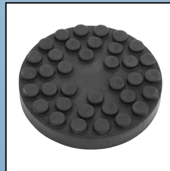
Rubber pad Ø145 mm for lift stabilizers SBR, black, SH 80 A Internal height 26 mm
