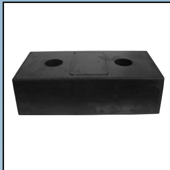
Buffer, vulcanized new rubber with vulcanized steel washers 500 x 250 x 140 mm
